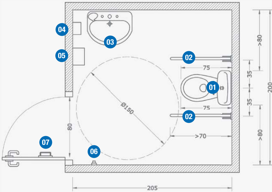
03 Lavamanos Handwash Ref. GW11 49 07 00
