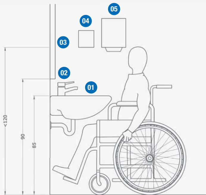
Lavamanos Handwash Ref. GW11 49 07 00
