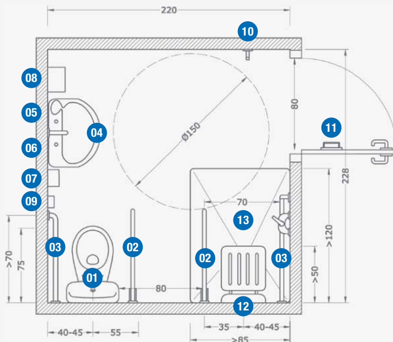
Barra abatible Folding bar Ref. GW11 07 04 01
