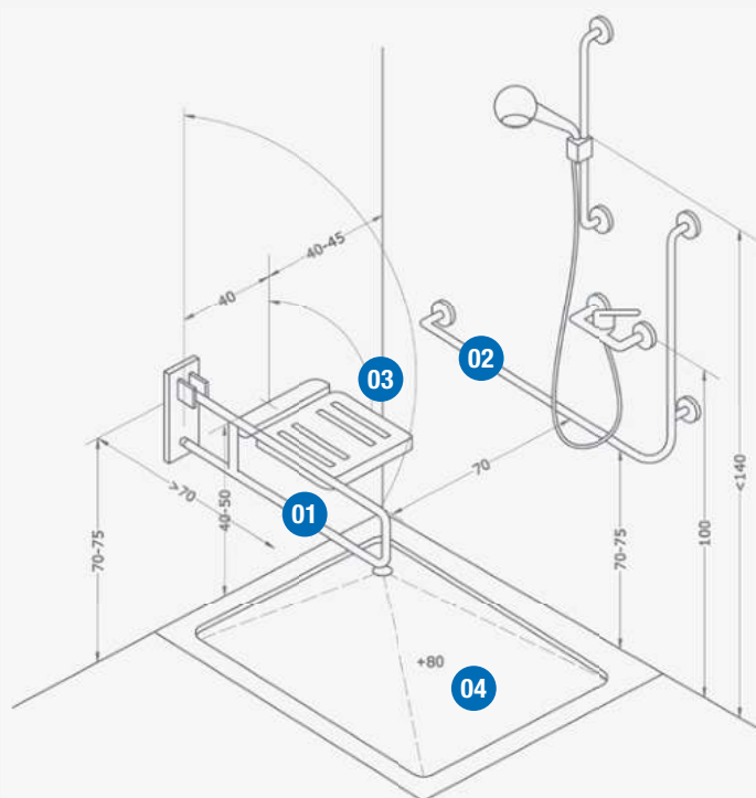
Barra abatible Folding bar Ref. GW11 07 04 01
