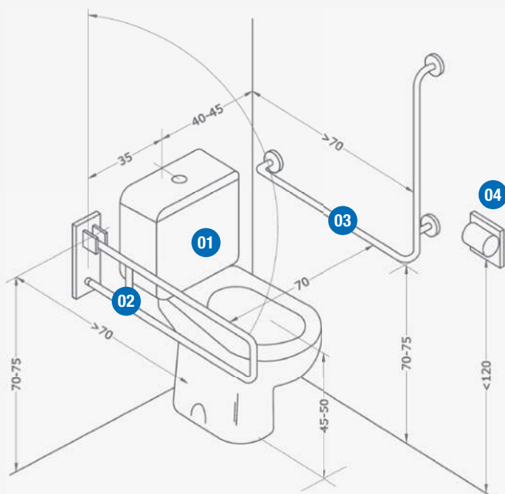
WC ergonómico Ergonomic WC Ref. GW11 42 07 00
